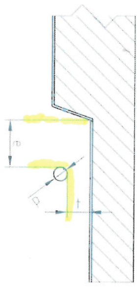
Detail X
